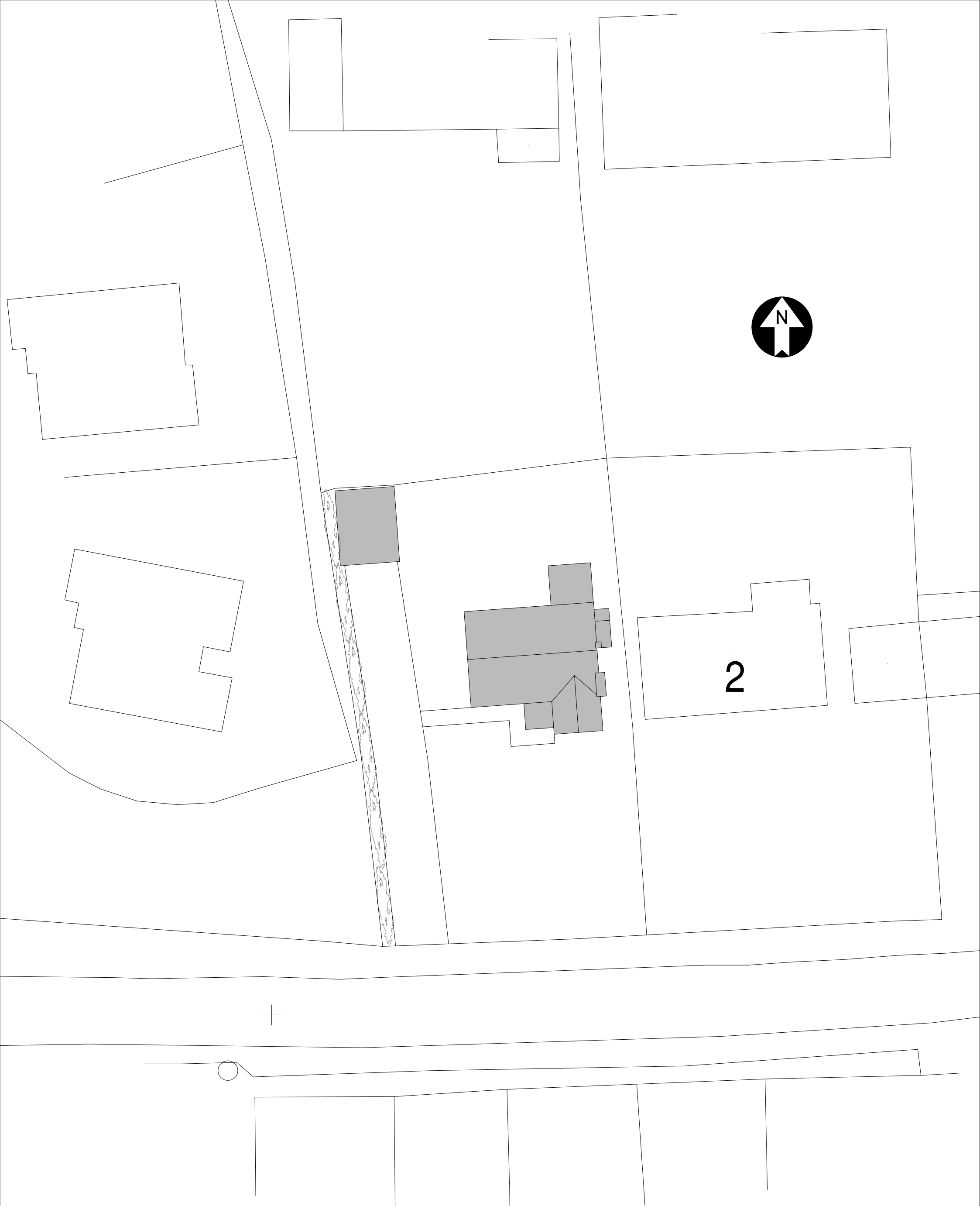
Existing Site Plan (scale 1:250@A3)
